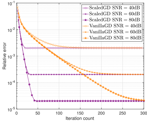
(b) Robust PCA n = 1000, r = 10, \alpha = 0.1
