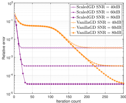
(c) Matrix completion n = 1000, r = 10, p = 0.2
