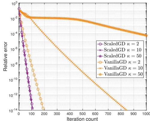
Figure 1: Performance of ScaledGD and vanilla GD for completing a 1000 \times 1000 incoherent matrix of rank 10 with different condition numbers \kappa = 2, 10, 50 , where each entry is observed independently with probability 0.2. Here, both methods are initialized via the spectral method. It can be seen that ScaledGD converges much faster than vanilla GD even for moderately large condition numbers.
