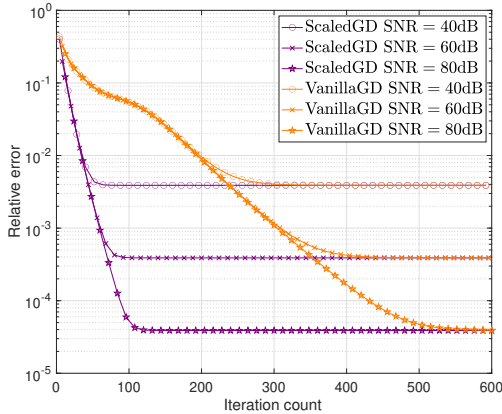
(a) Matrix Sensing n = 200, r = 10, m = 5nr
