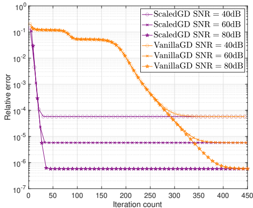
(d) Hankel matrix completion n = 1000, r = 10, p = 0.2
