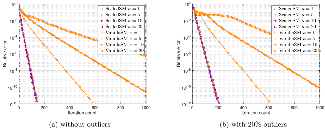
Figure 2: Performance comparisons of ScaledSM and VanillaSM for quadratic sensing without or with outliers under different condition numbers \kappa = 1, 5, 10, 20 , where n = 100 , r = 5 , and m = 8nr .
