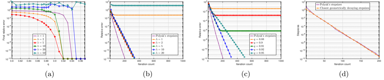
Figure 6: Performance comparisons of ScaledSM for quadratic sensing using the geometrically decaying stepsize with parameters (\lambda, q) and Polyak’s stepsize, where we fix n = 100 , r = 5 , m = 8nr , \kappa = 10 , and p_s = 0.2 : (a) the final relative error for various combinations of (\lambda, q) , (b) the relative error versus iteration count for fixed q = 0.92 and varying \lambda , (c) the relative error versus iteration count for fixed \lambda = 2 and varying q , and (d) shows a properly tuned geometrically decaying stepsize with \lambda = 1.36 and q = 0.88 essentially matches the performance of Polyak’s stepsize.
